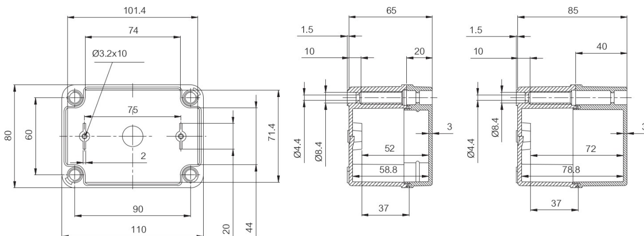
Illustration 5: Housing dimensions. Note: Drawing not including air inlet. Dimensions in mm.
