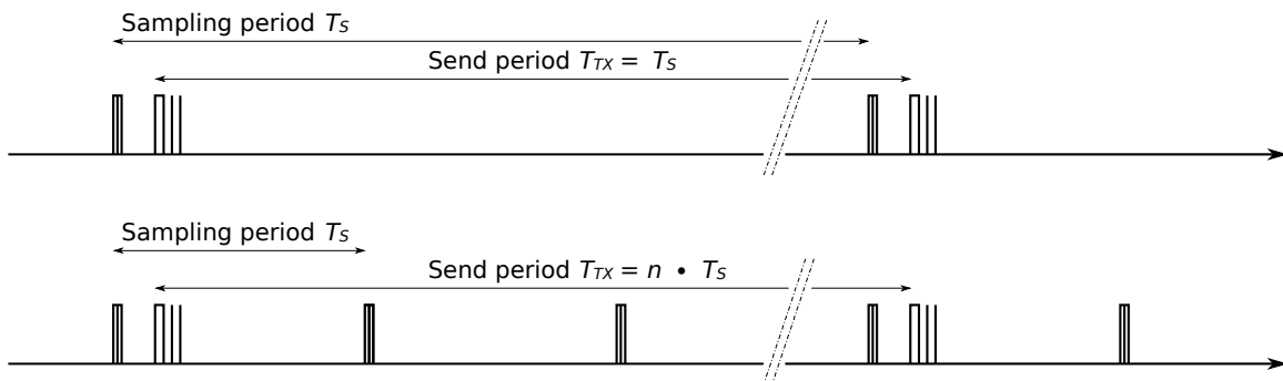
Illustration 4: Sampling period vs. send period shown for two configurations. Default for DL-LP8P: T_s = 1 \text{ min} , T_{TX} = 10 \cdot 1 \text{ min} (second row).
